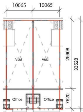
Intermediate lot 1st floor plan
