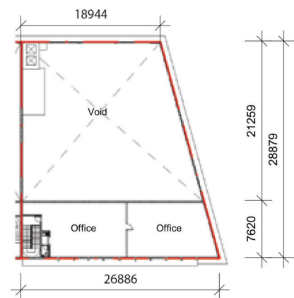
D11 (Corner lot) 1st floor plan
