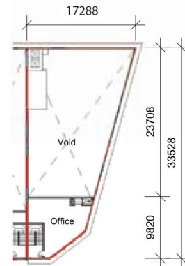
C12 (Corner lot) 1st floor plan
