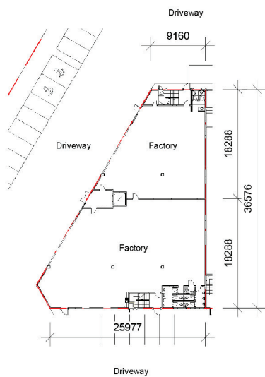
B1 (Corner lot) Ground floor plan
