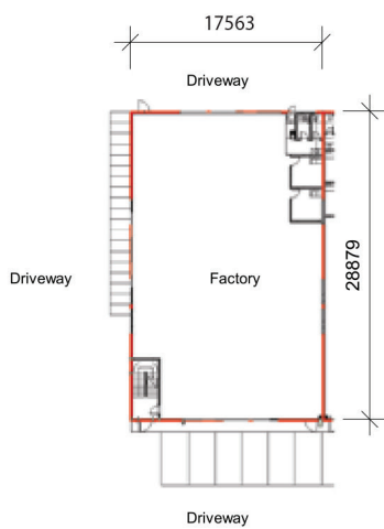
D1 (Corner lot) Ground floor plan
