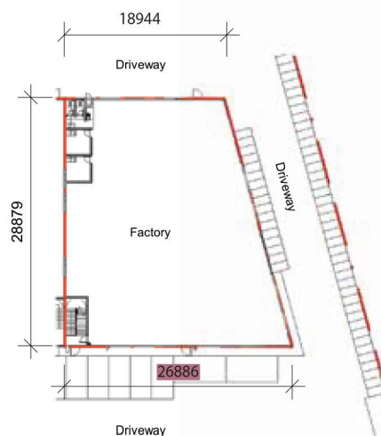
D11 (Corner lot) Ground floor plan
