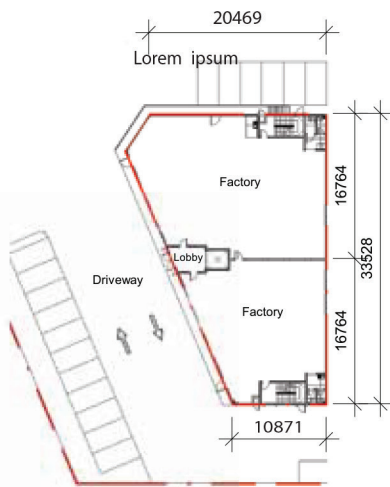
A1 (Corner lot) Ground floor plan
