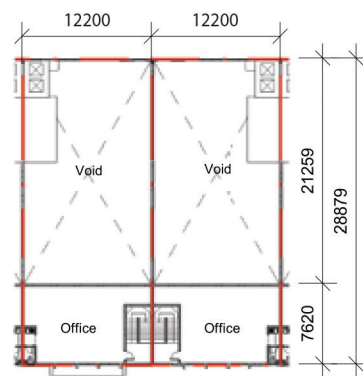
Intermediate lot 1st floor plan
