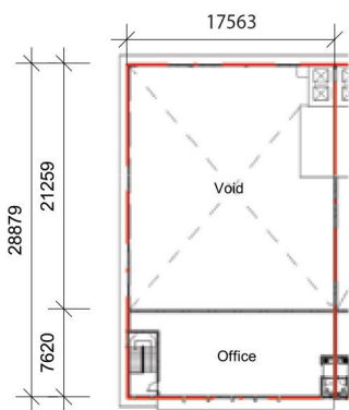
D1 (Corner lot) 1st floor plan
