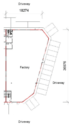
B10 (Corner lot) Ground floor plan
