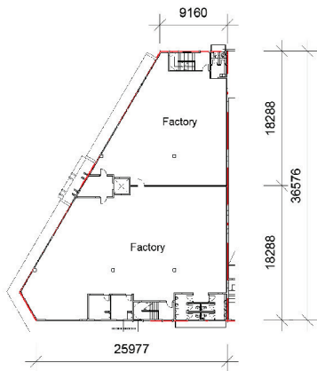
B1 (Corner lot) 1st floor plan
