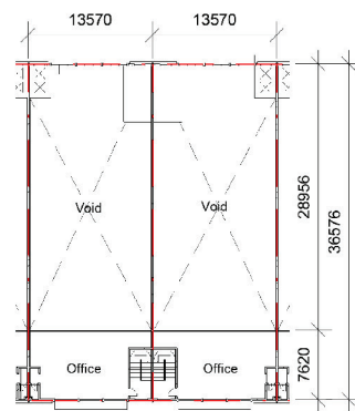
Intermediate lot 1st floor plan
