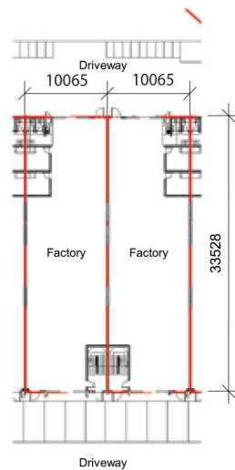
Intermediate lot 1st floor plan
