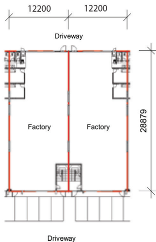
Intermediate lot Ground floor plan
