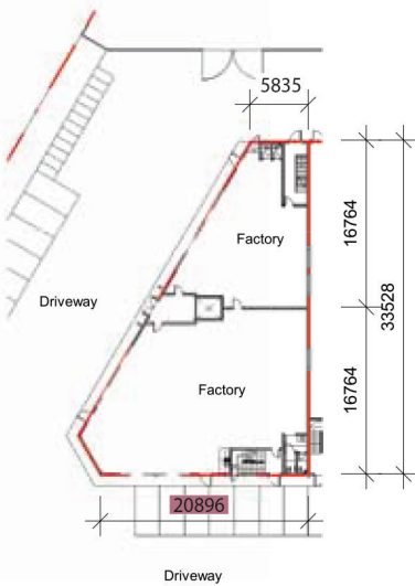
C1 (Corner lot) Ground floor plan
