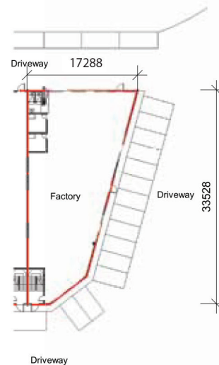
C12 (Corner lot) 1st floor plan
