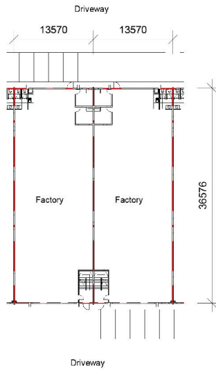
Intermediate lot Ground floor plan
