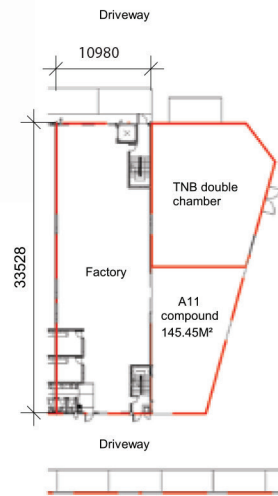
A11 (Corner lot) Ground floor plan
