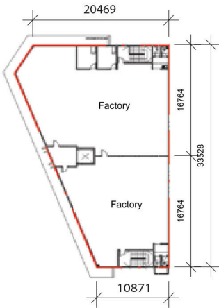
A1 (Corner lot) 1st floor plan
