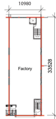
A11 (End lot) 1st floor plan
