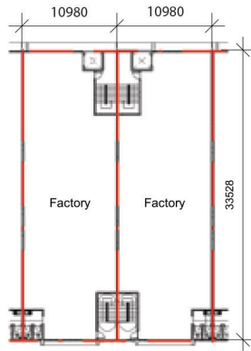
Intermediate lot 1st floor plan
