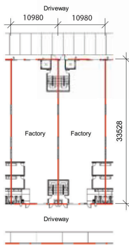
Intermediate lot Ground floor plan
