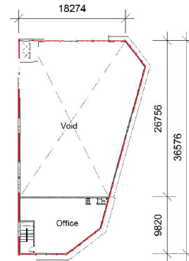
B10 (Corner lot) 1st floor plan
